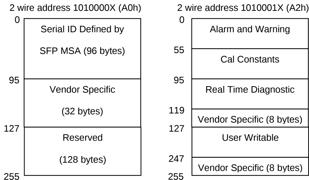
Fig 2 EEPROM Information
