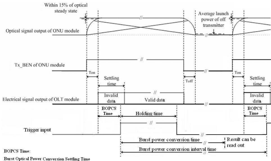
Figure2 Trigger sequence definition in GPON system
